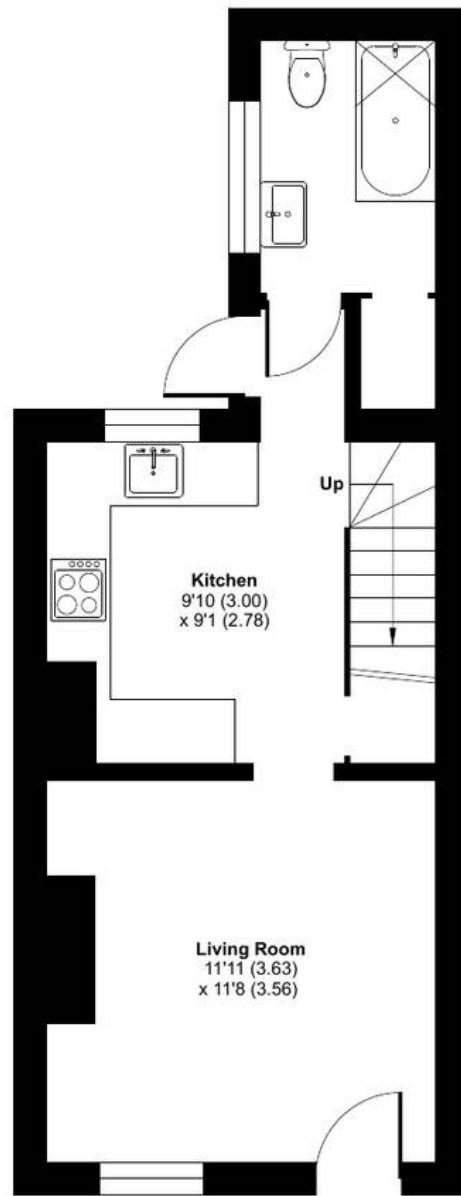
GROUND FLOOR
