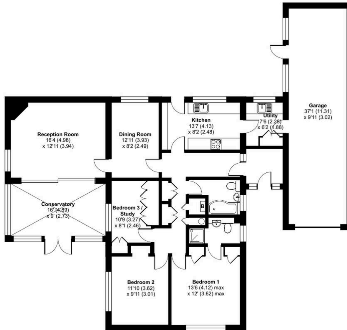
GROUND FLOOR
